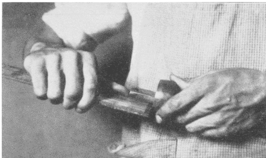
Fig. 213. Setting a Marking-Gage.
