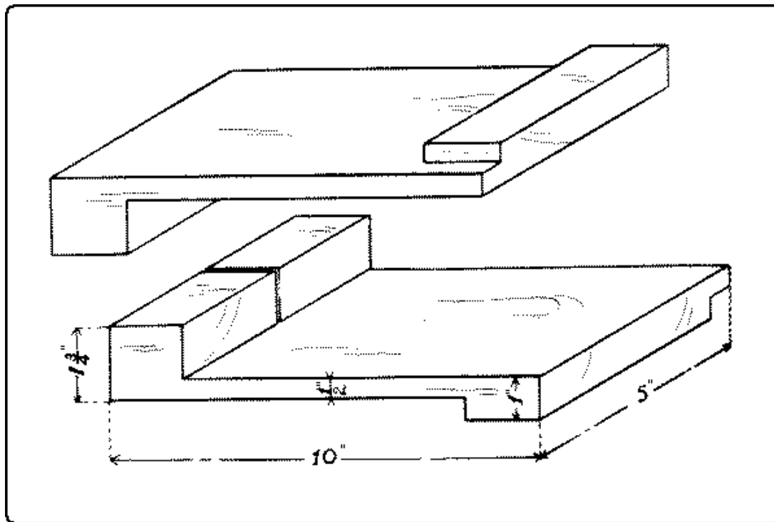
Fig. 179. Bench-Hook.
