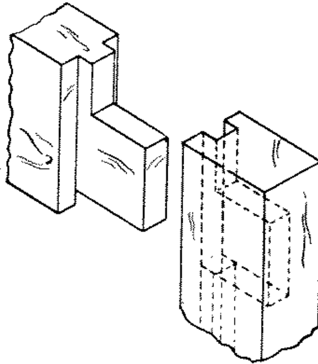
Fig. 267-42 Haunched mortise and tenon
