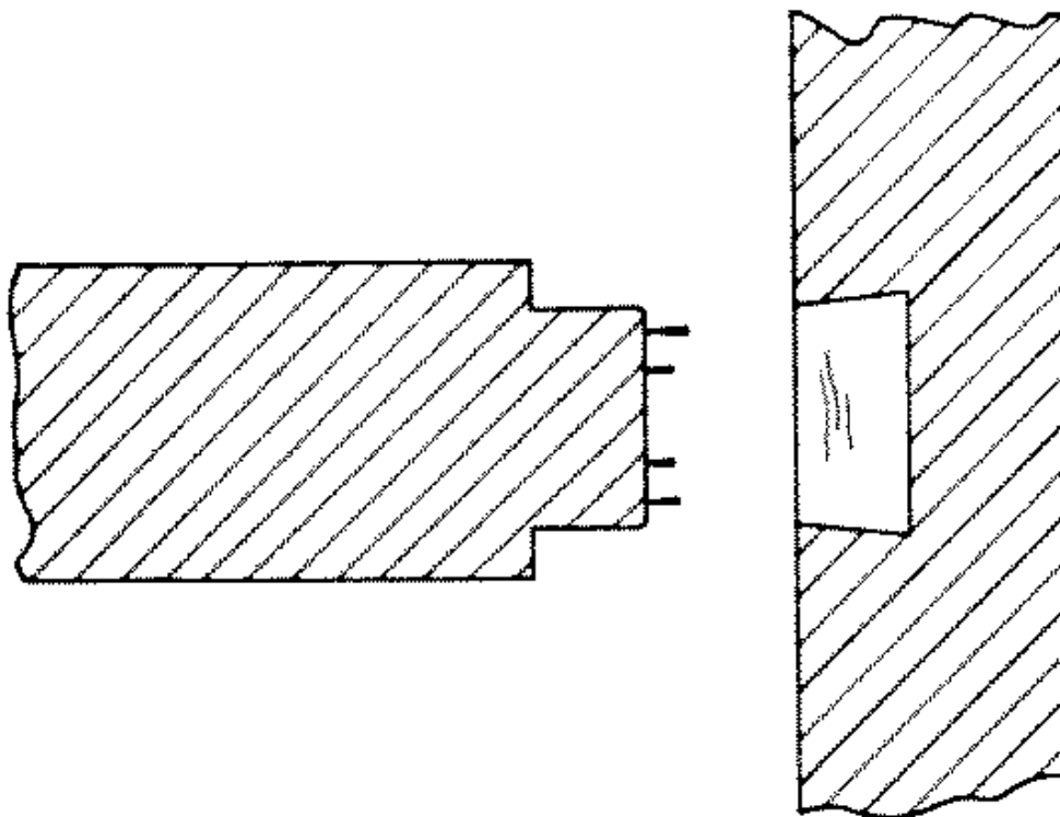
Fig. 266-36 Fox tail tenon
