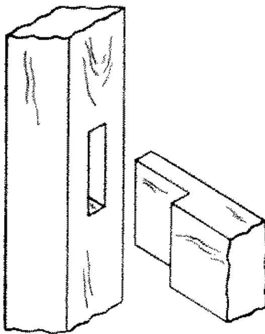
Fig. 267-44 Bare faced tenon
