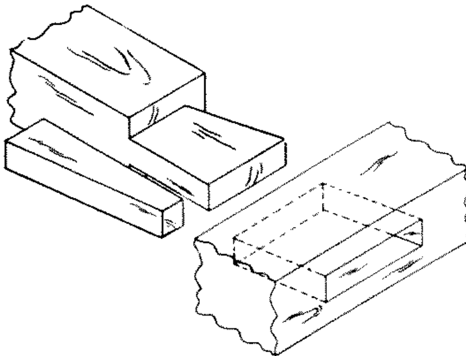
Fig. 266-37 Dovetail mortise and tenon
