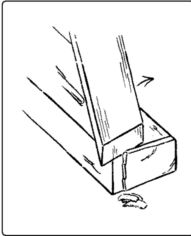
Fig. 73. Chiseling End Wood.
