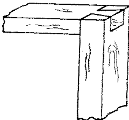
Fig. 267-47 Thru single dovetail
