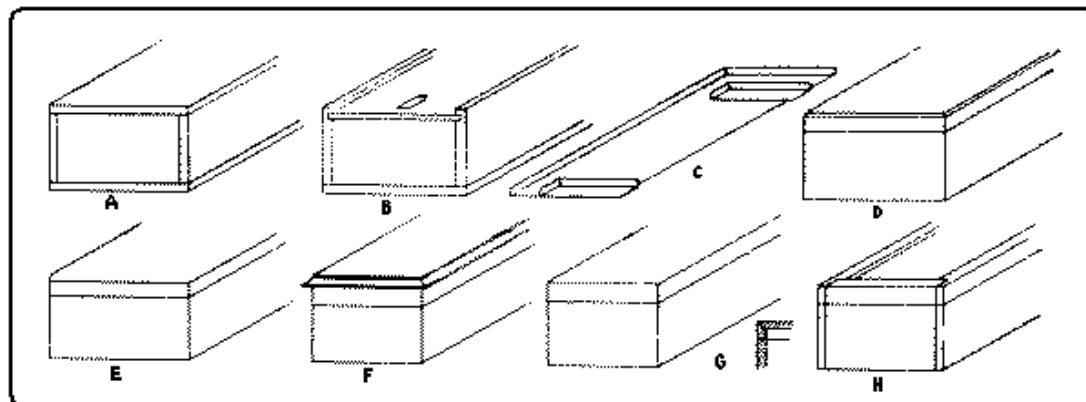
Fig. 285. Forms of Box Construction.
