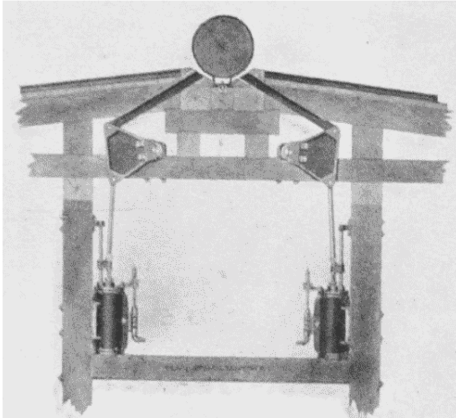
Fig. 38. Log-Flipper.
