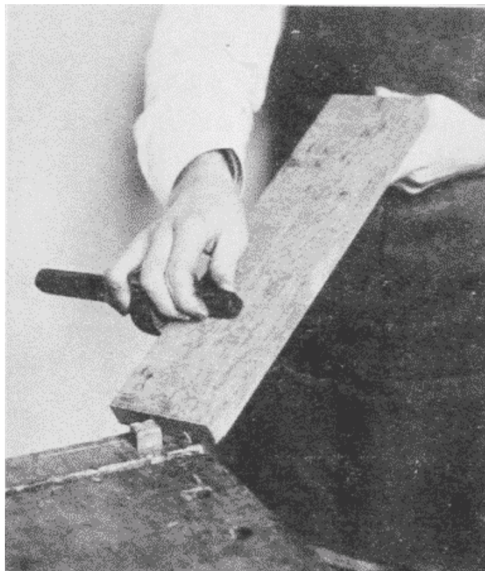
Fig. 214. Using the Marking-Gage.
