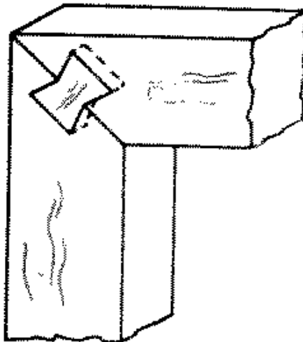
Fig. 268-57 Double dovetail keyed
