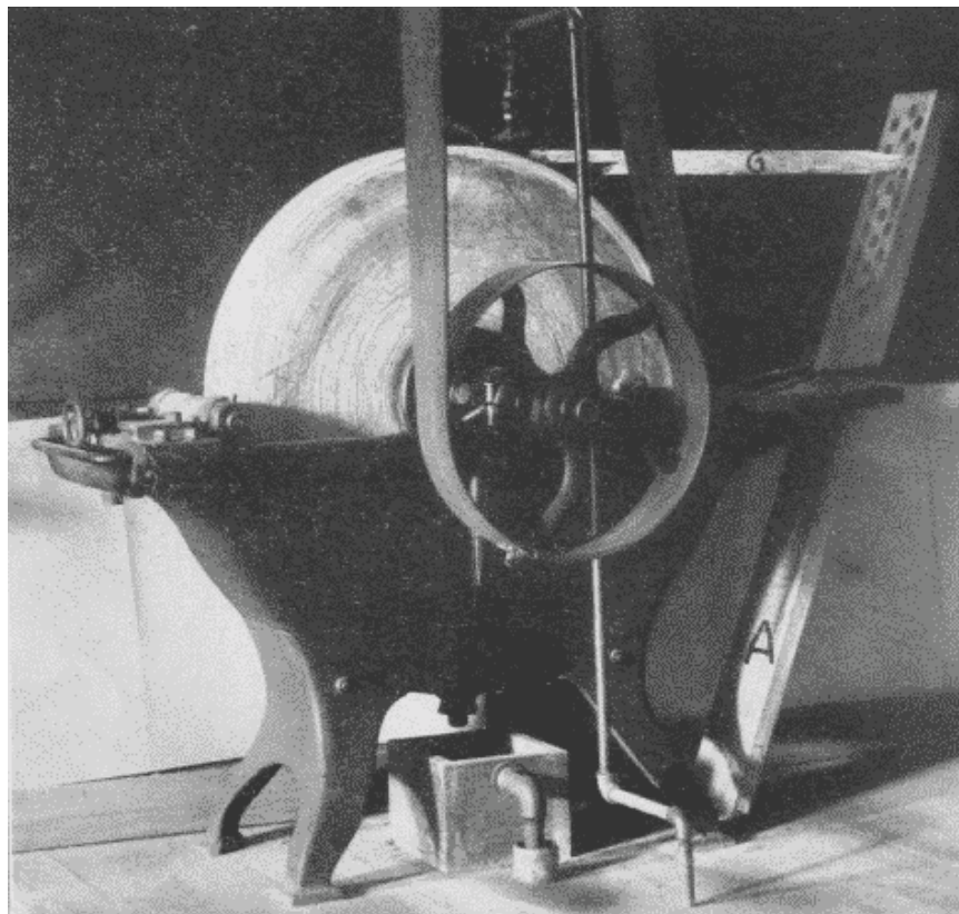
Fig. 221. Power Grindstone.
