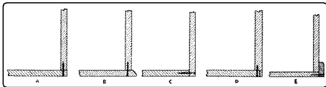
Fig. 284. Methods of Attaching Box Bottoms.
