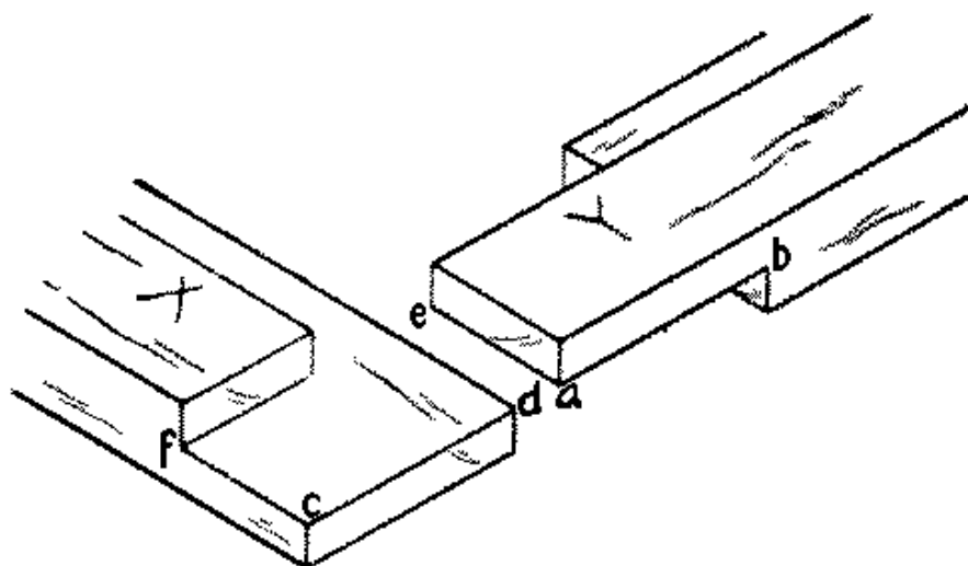
Fig. 265-17 End lap with rabbet
