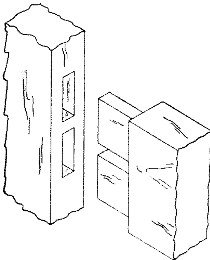
Fig. 267-41 Double mortise and tenon
