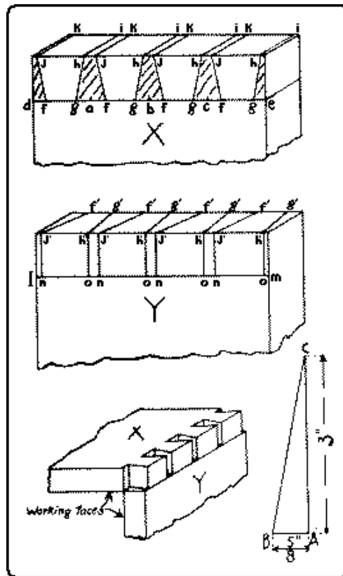
Fig. 250. Laying Out a Dovetail Joint.
