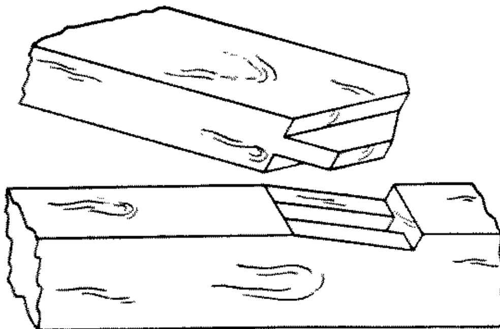
Fig. 269-67 Oblique mortise and tenon
