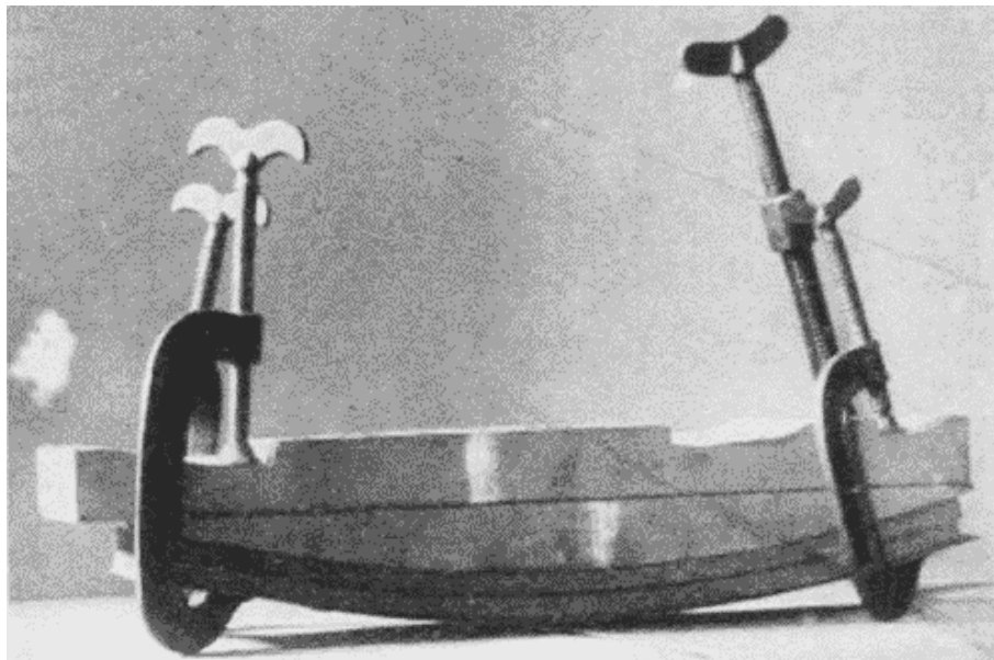
Fig. 299. Bending Boards into Shape after Boiling Them.
