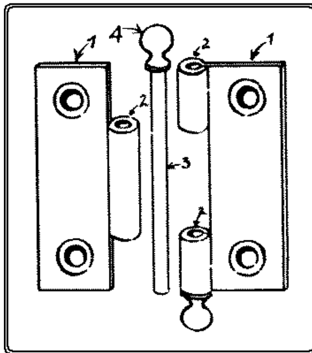
Fig. 234. Parts of a butt-hinge.
