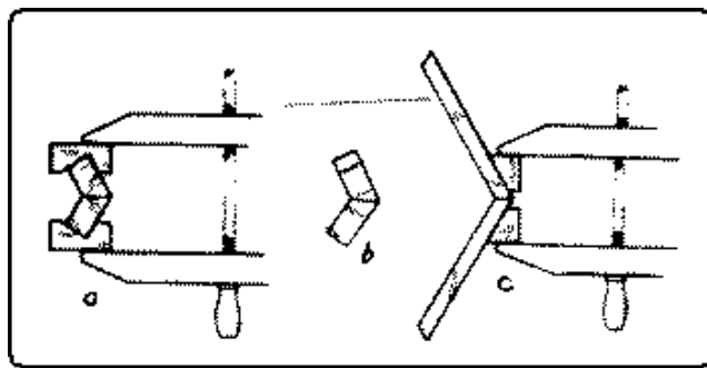
Fig. 258. Devices for Gluing Beveled Edges.
