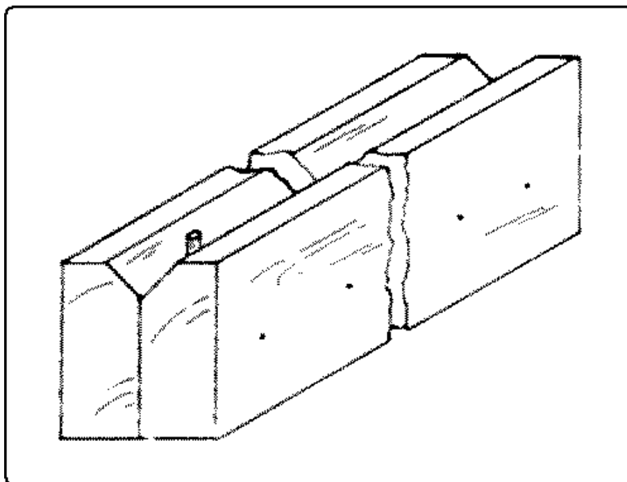
Fig. 274. Trough for Planing Chamfers.
