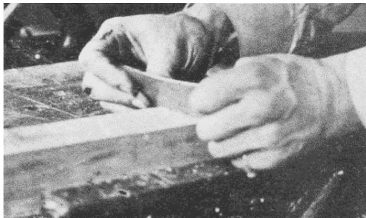
Fig. 152. Using a Cabinet-Scraper.
