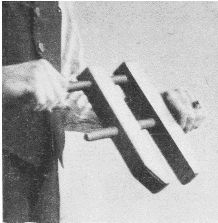
Fig. 174. Adjusting Handscrew.
