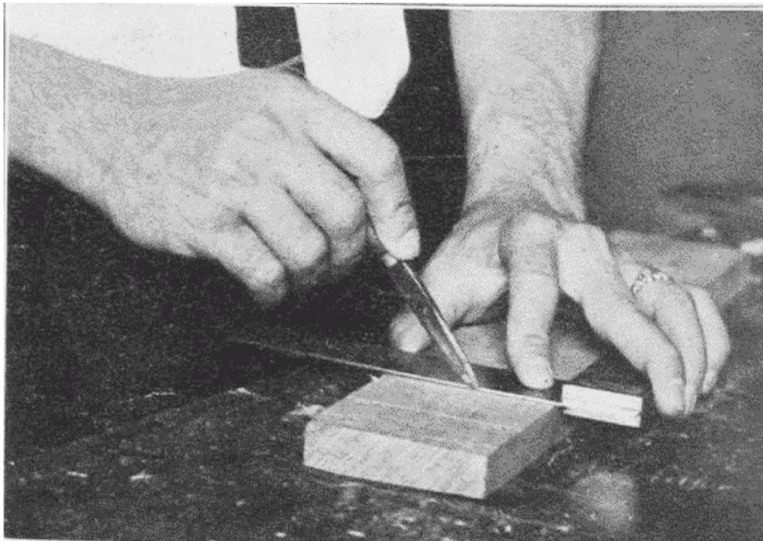
Fig. 204. Scribing with Knife by Try-Square.
