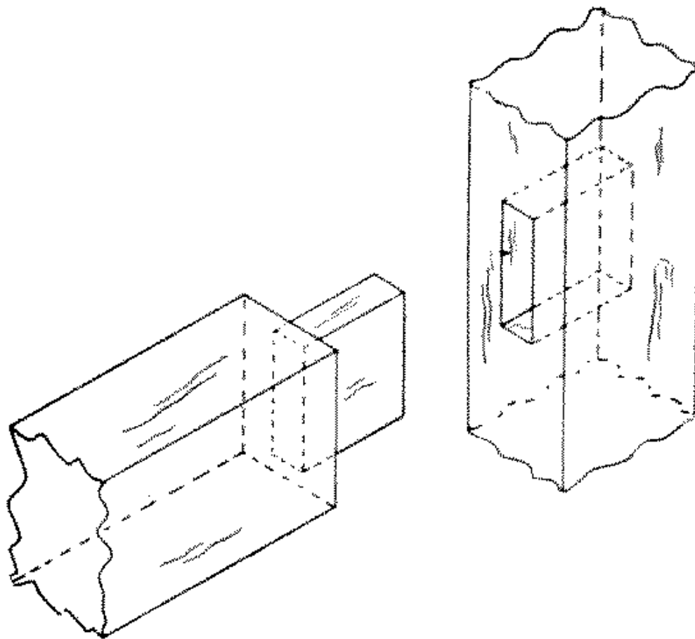
Fig. 266-32 Blind mortise and tenon
