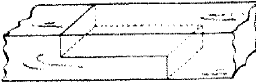
Fig. 264-4 Spliced for compression
