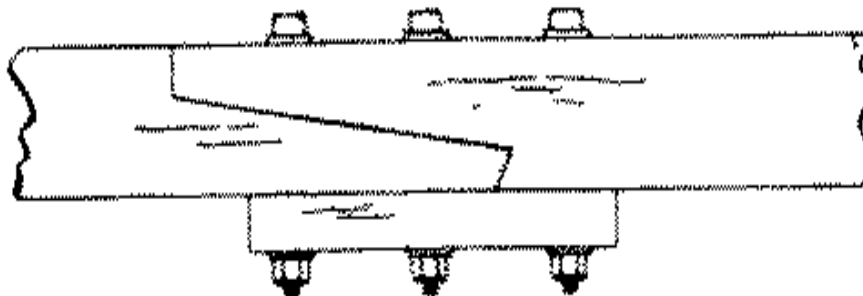
Fig. 264-7 Spliced for cross strain
