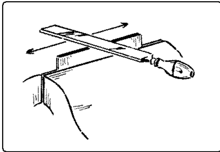
Fig. 153. Sharpening a Cabinet-Scraper: 1st Step, Drawfiling.
