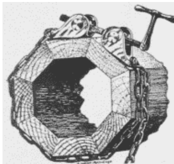
Fig. 259. Column-Clamp.
