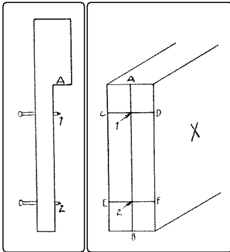
Fig. 249. Laying out a Dowel Joint.
