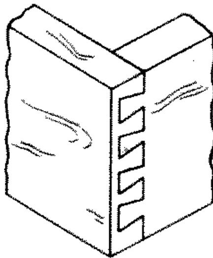
Fig. 267-49 Lap dovetail
