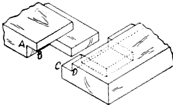
Fig. 266-33 Mortise and tenon with rabbet
