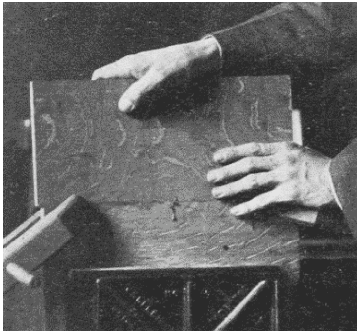
Fig. 261. Rubbing a Glued Joint.
