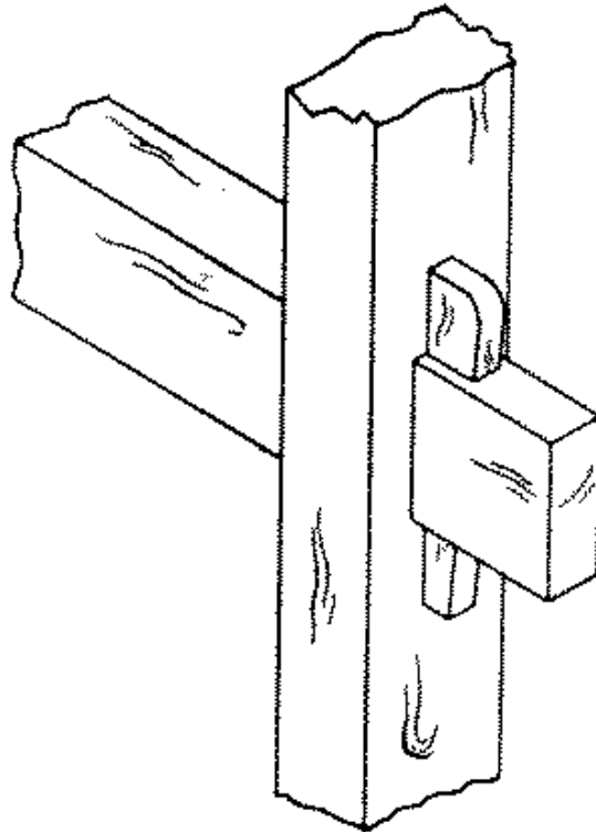
Fig. 267-39 Keyed mortise and tenon
