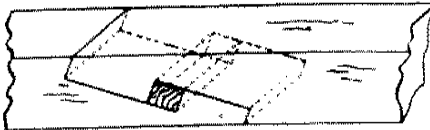
Fig. 264-5 Spliced for tension
