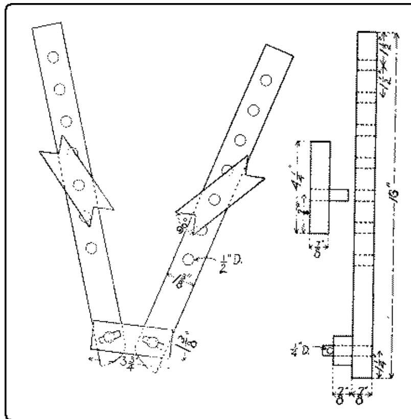
Fig. 255. Picture-Frame-Clamp. (See also Fig. 254.)
