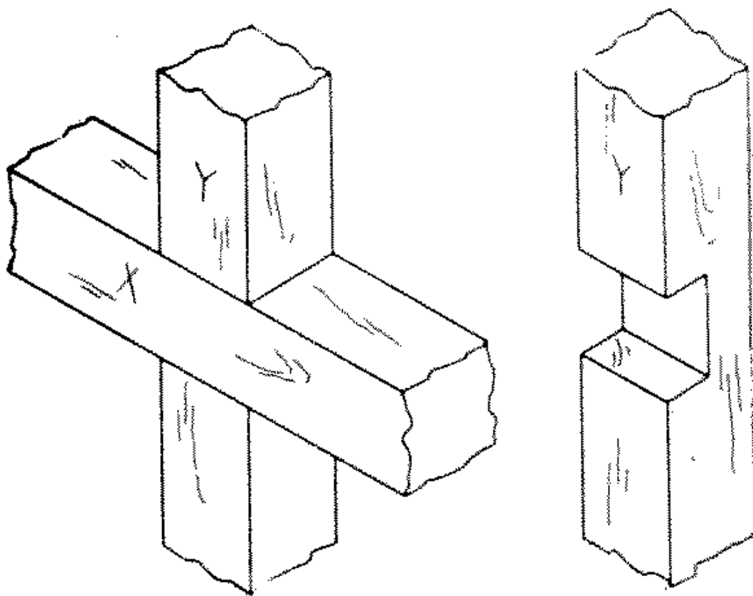
Fig. 264-14 Cross lap
