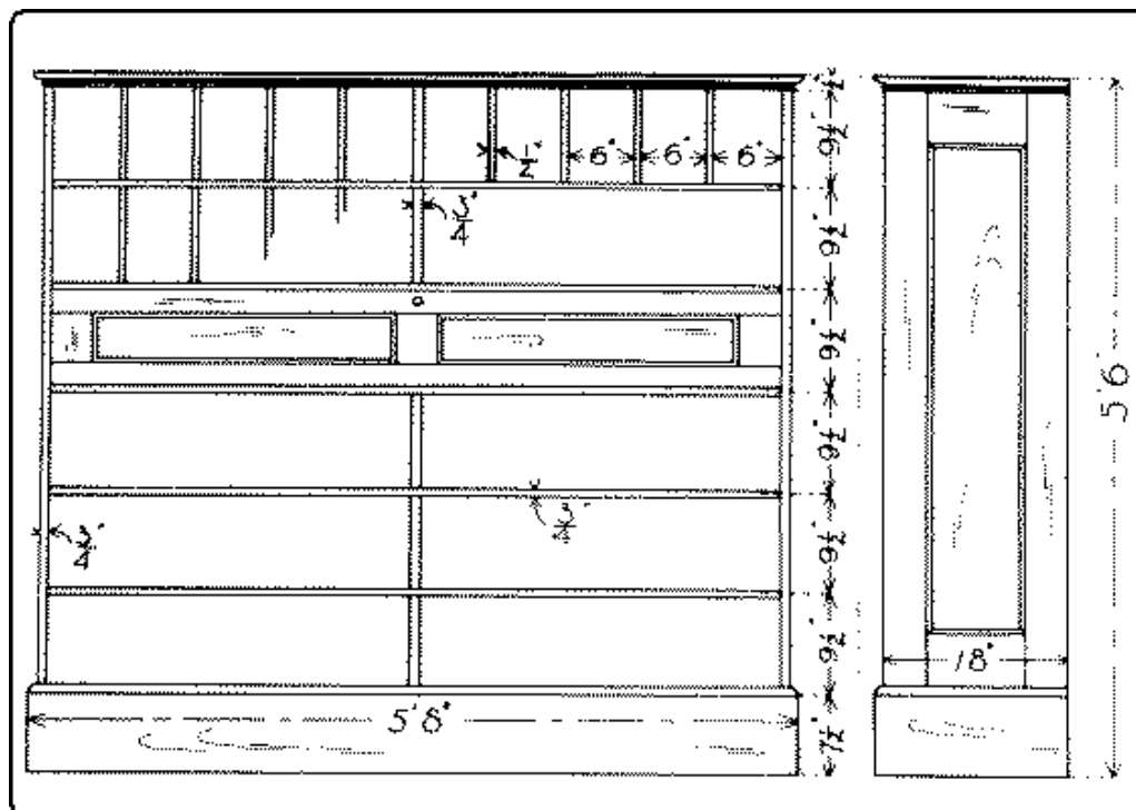
Fig. 242. A More Expensive Locker for Unfinished Work.
