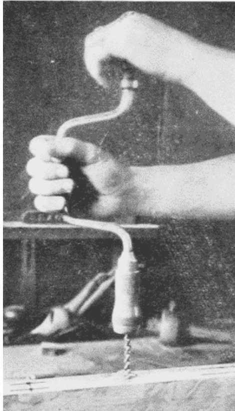
Fig. 263. Boring for Dowels in an Edge-to-Edge Joint.
