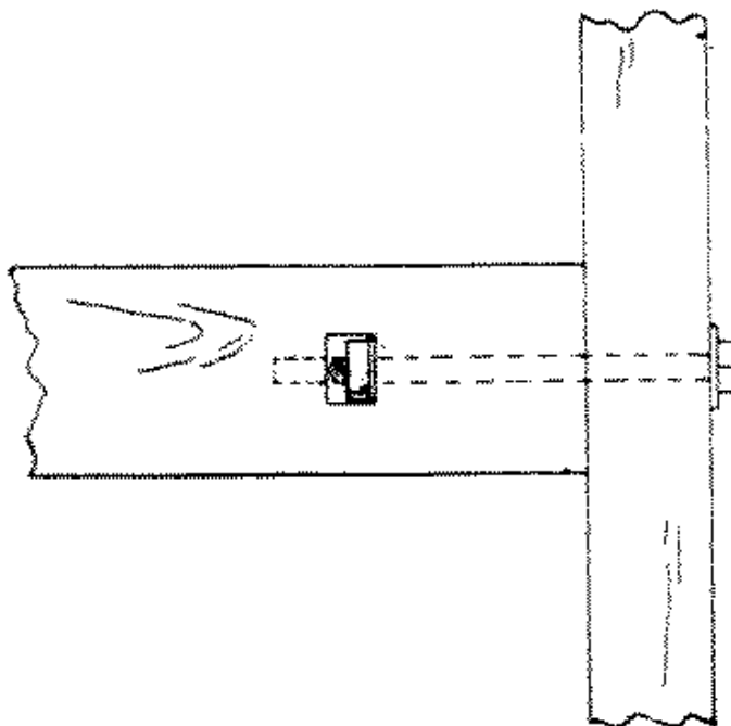
Fig. 264-10 Draw-bolt
