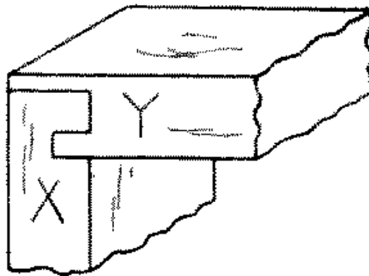
Fig. 266-27 Dado tongue and rabbet
