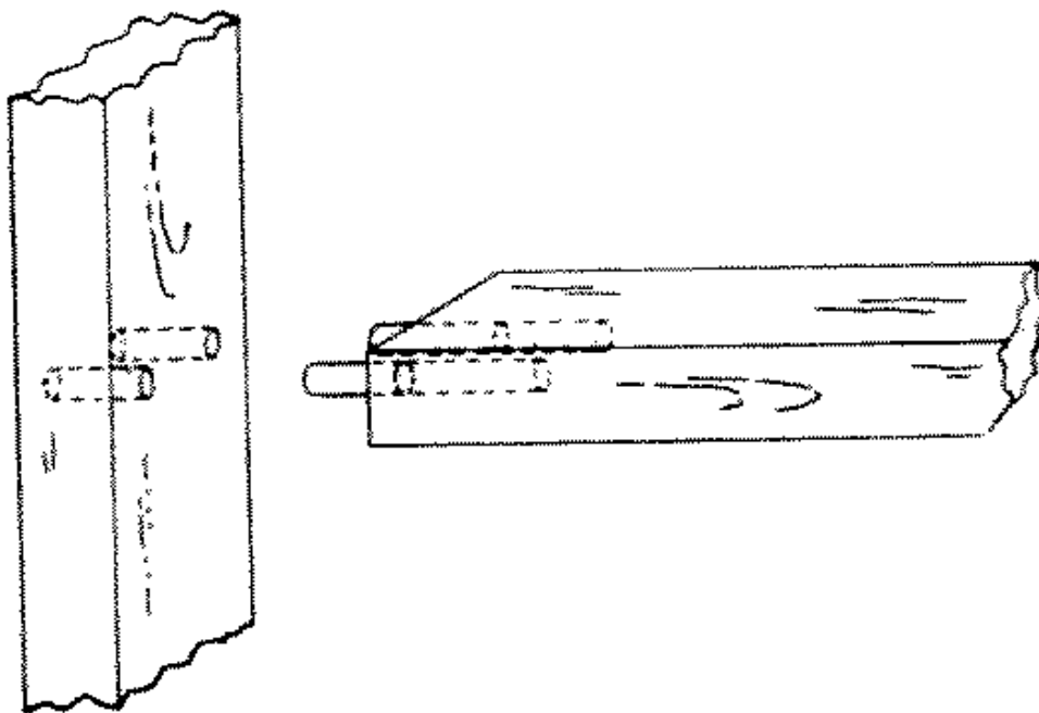
Fig. 264-8 Doweled butt
