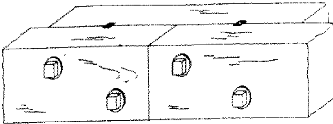
Fig. 264-3 Fished and keyed
