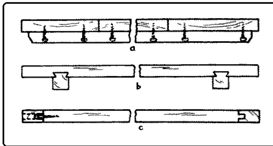
Fig. 280. Drawing-Board Construction:
