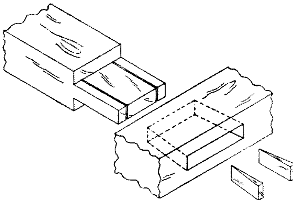
Fig. 266-35 Wedged mortise and tenon
