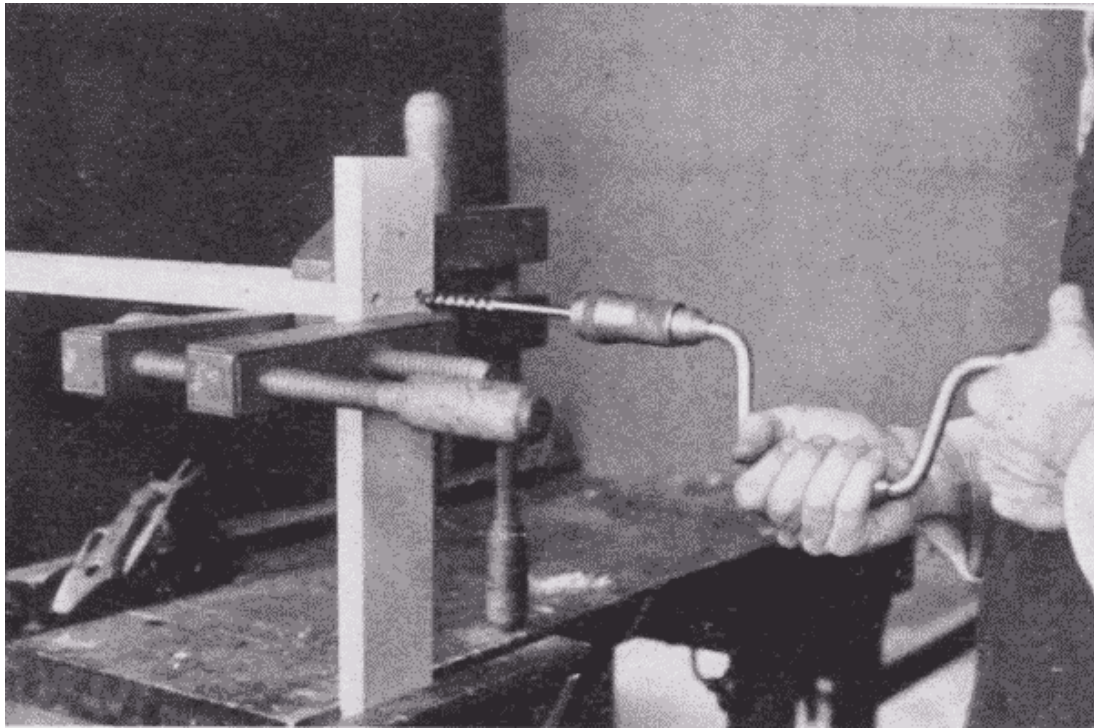
Fig. 247. Thru Boring for a Butt Joint.
