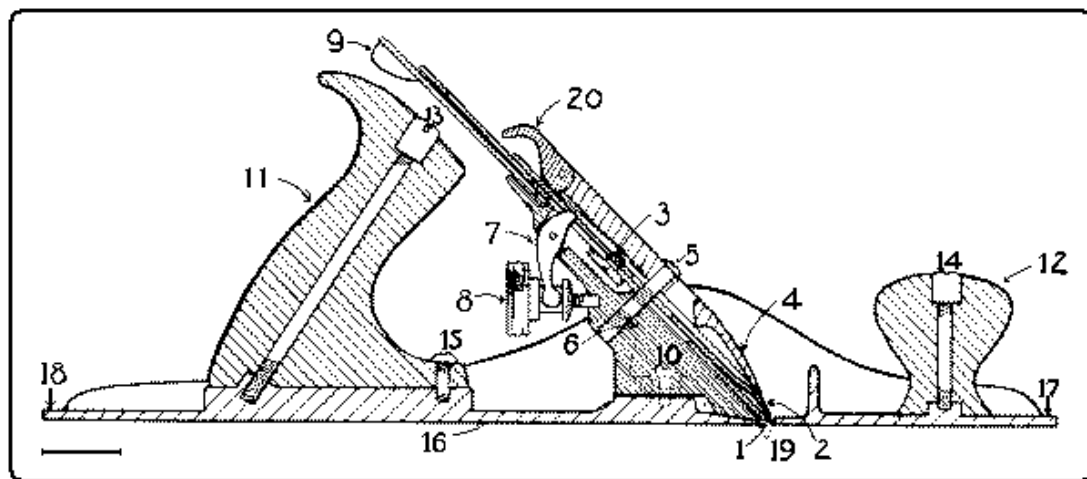
Fig. 101 Section of Jack Plane.
