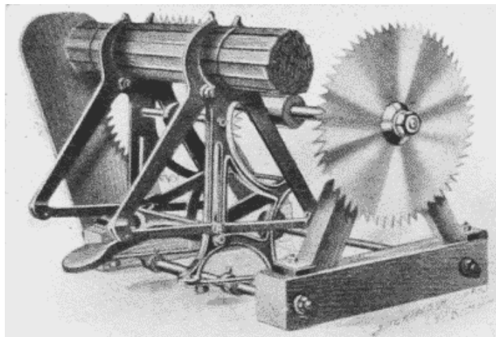
Fig. 51. Combination Lath-Binder and Trimmer. With this machine the operator can trim the bundles of lath simply by tilting the packing
