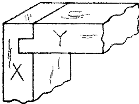
Fig. 266-26 Dado and rabbet
