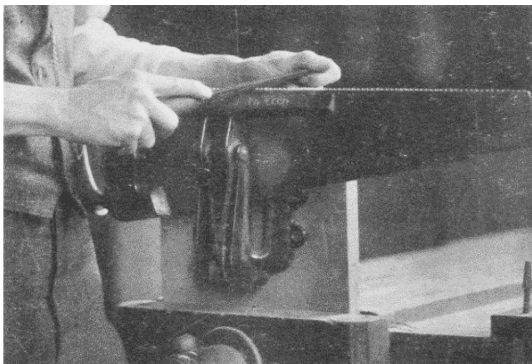
Fig. 96. Saw-Vise.
