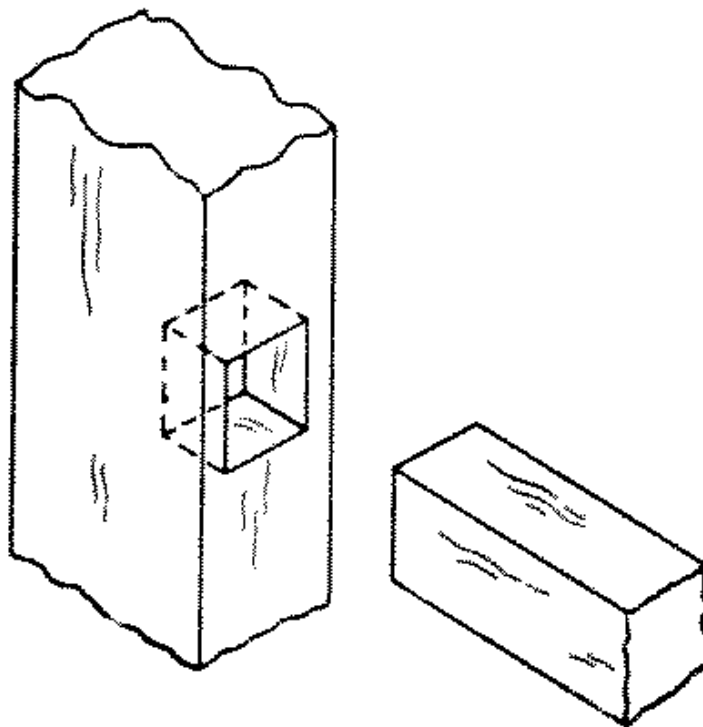
Fig. 267-45 Housed mortise and tenon
