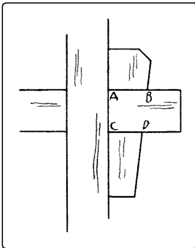
Fig. 252. Keyed Mortise-and-Tenon Joint.
