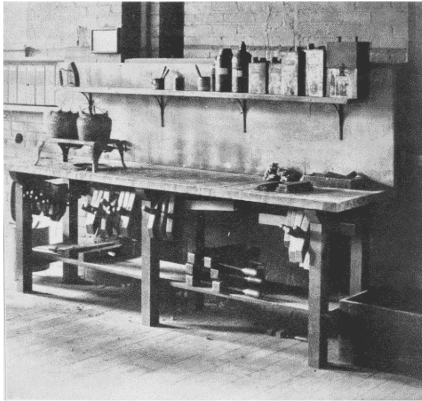
Fig. 243. Gluing and Staining Bench Covered with Zinc.
