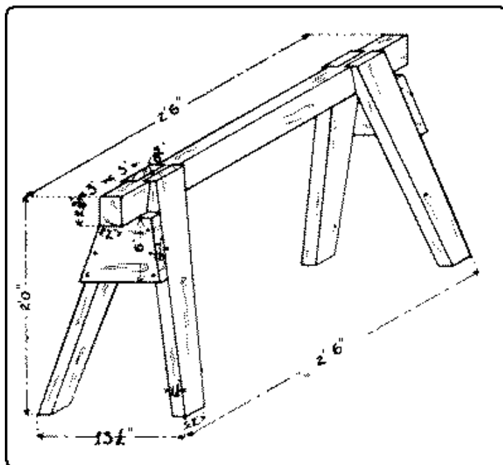
Fig. 170. Saw-Horse.
