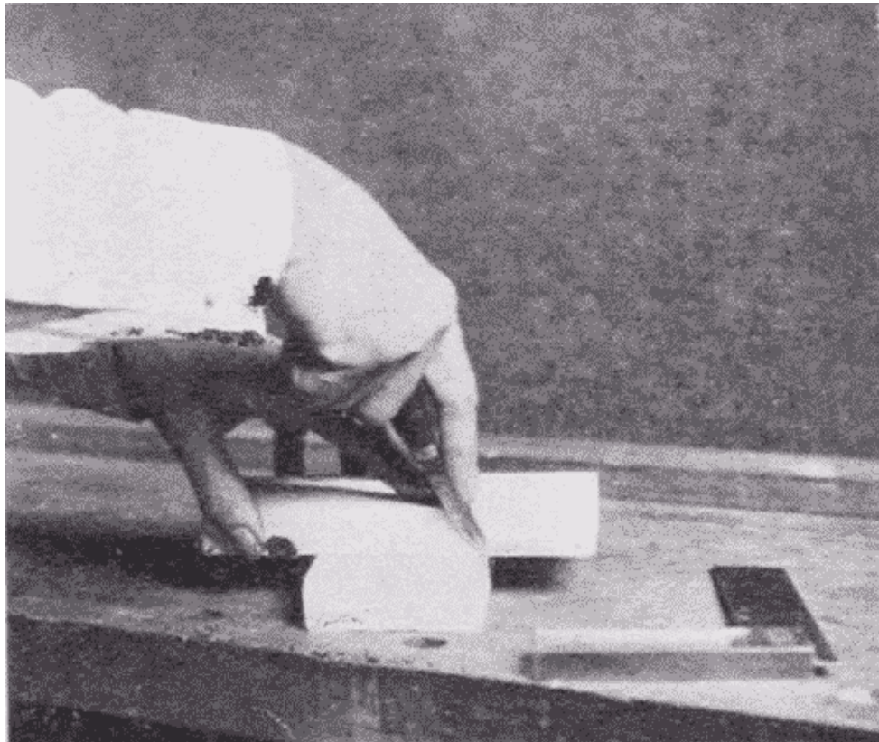
Fig. 302. Marking by Superposition.
