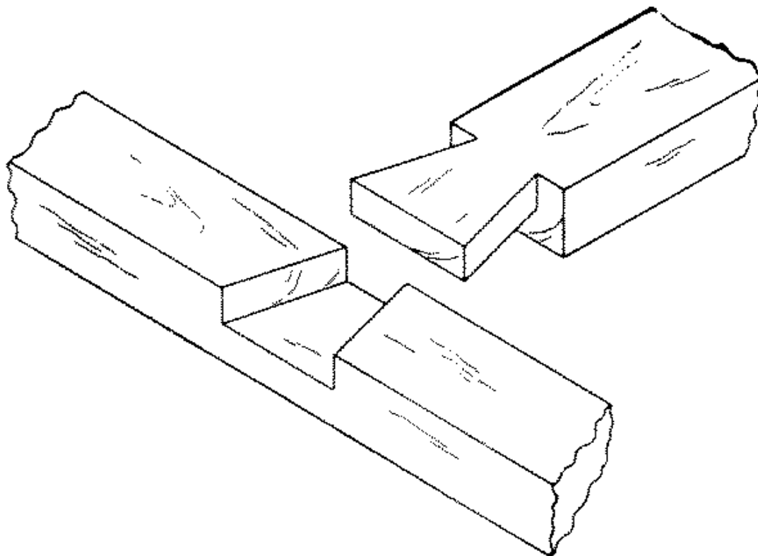
Fig. 265-18 Dovetail halving
