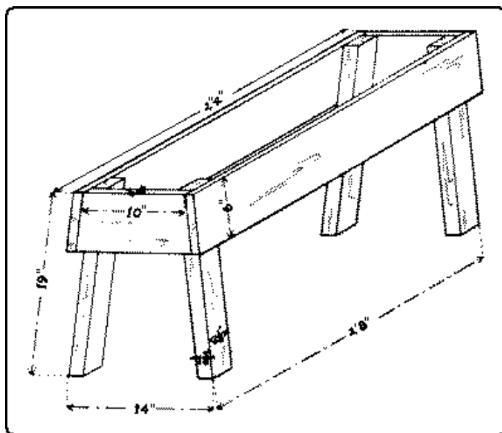
Fig. 171. Saw-Horse.
