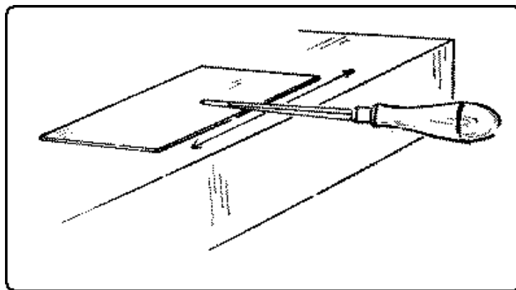
Fig. 157. Resharpening a Cabinet-Scraper: Flattening the Edge.
