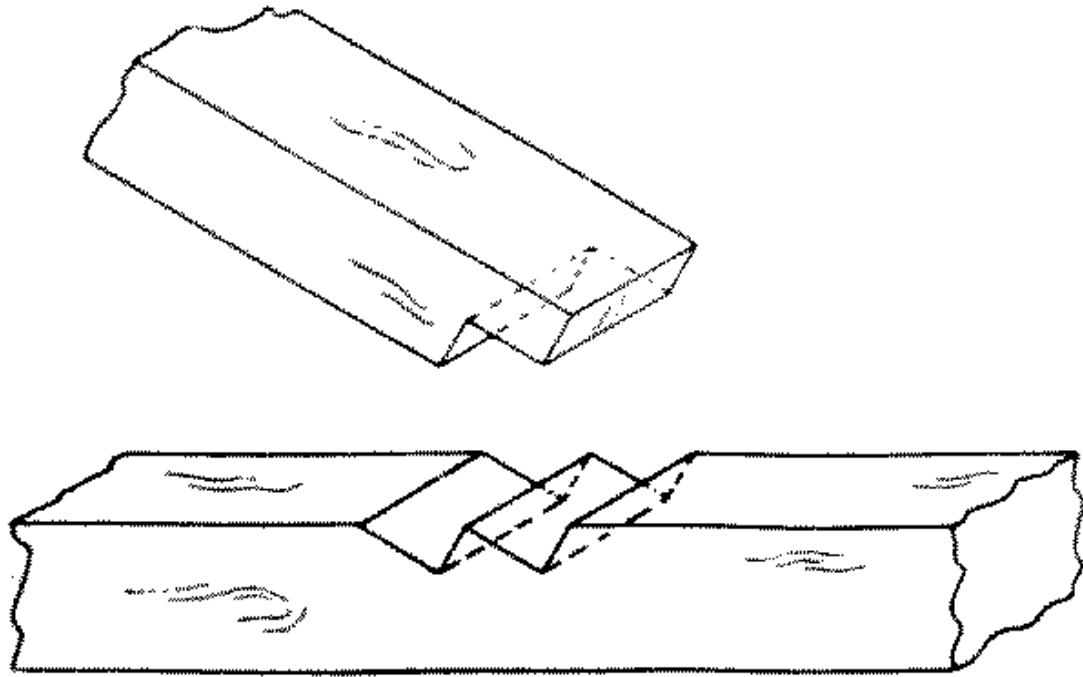
Fig. 268-63 Square thrust
