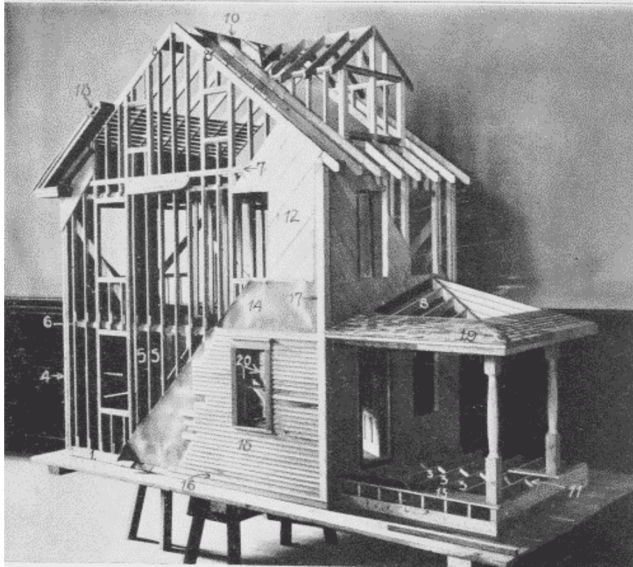
Fig. 300. House Construction.
