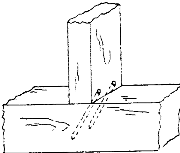
Fig. 264-9 Toe-nailed
