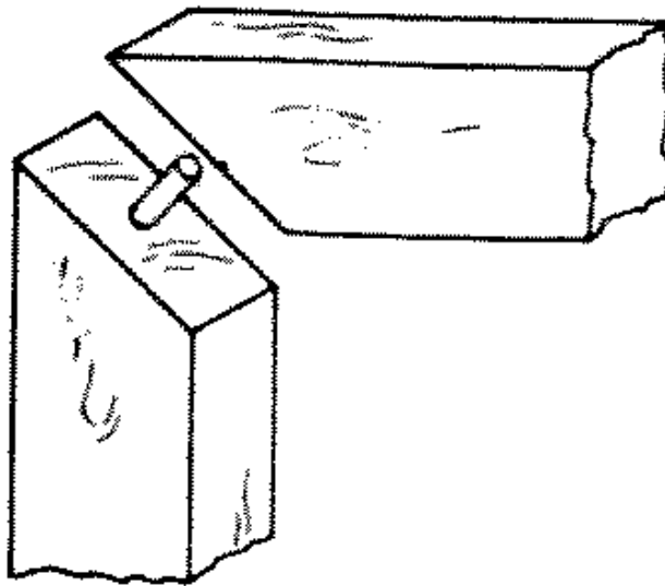
Fig. 268-53 Doweled miter
