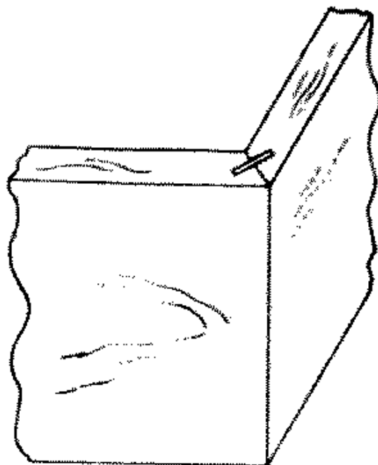
Fig. 268-54 Spline miter
