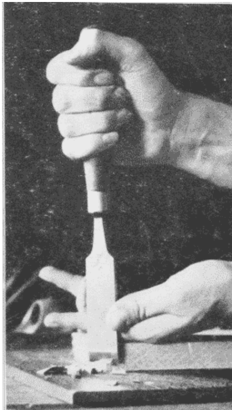
Fig. 72. Perpendicular Chiseling.
