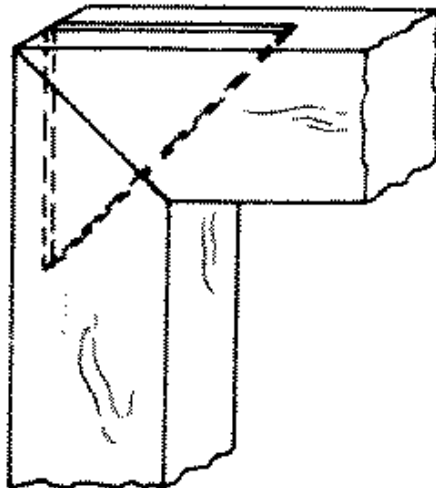
Fig. 268-55 Slip feather miter
