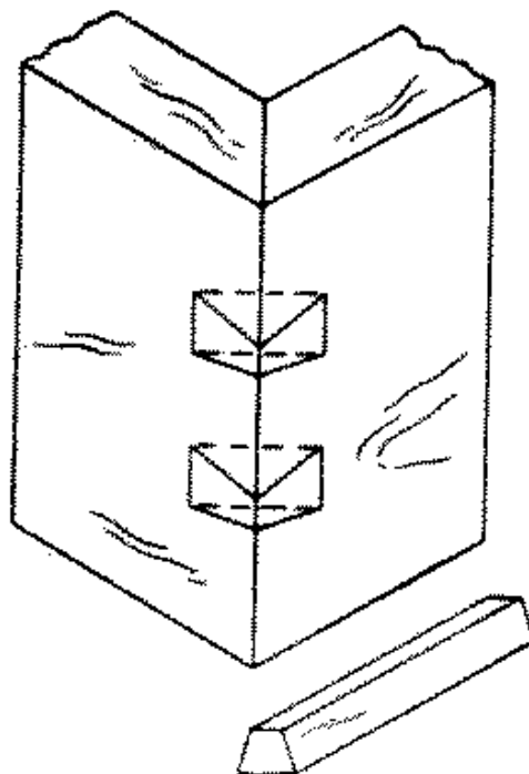
Fig. 268-56 Slip dovetail miter
