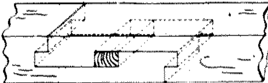
Fig. 264-6 Spliced and Tabled
