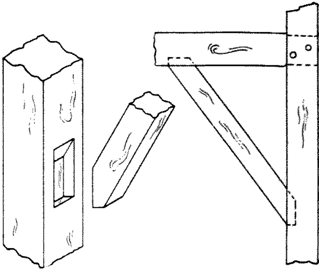
Fig. 269-66 Housed brace
