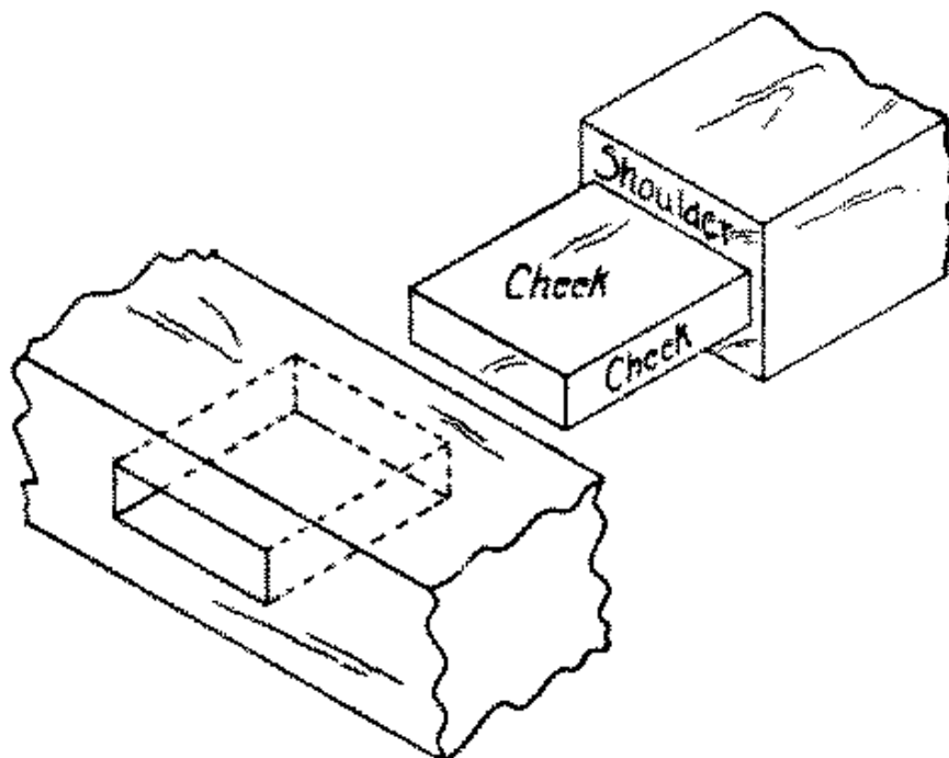
Fig. 266-31 Thru mortise and tenon
