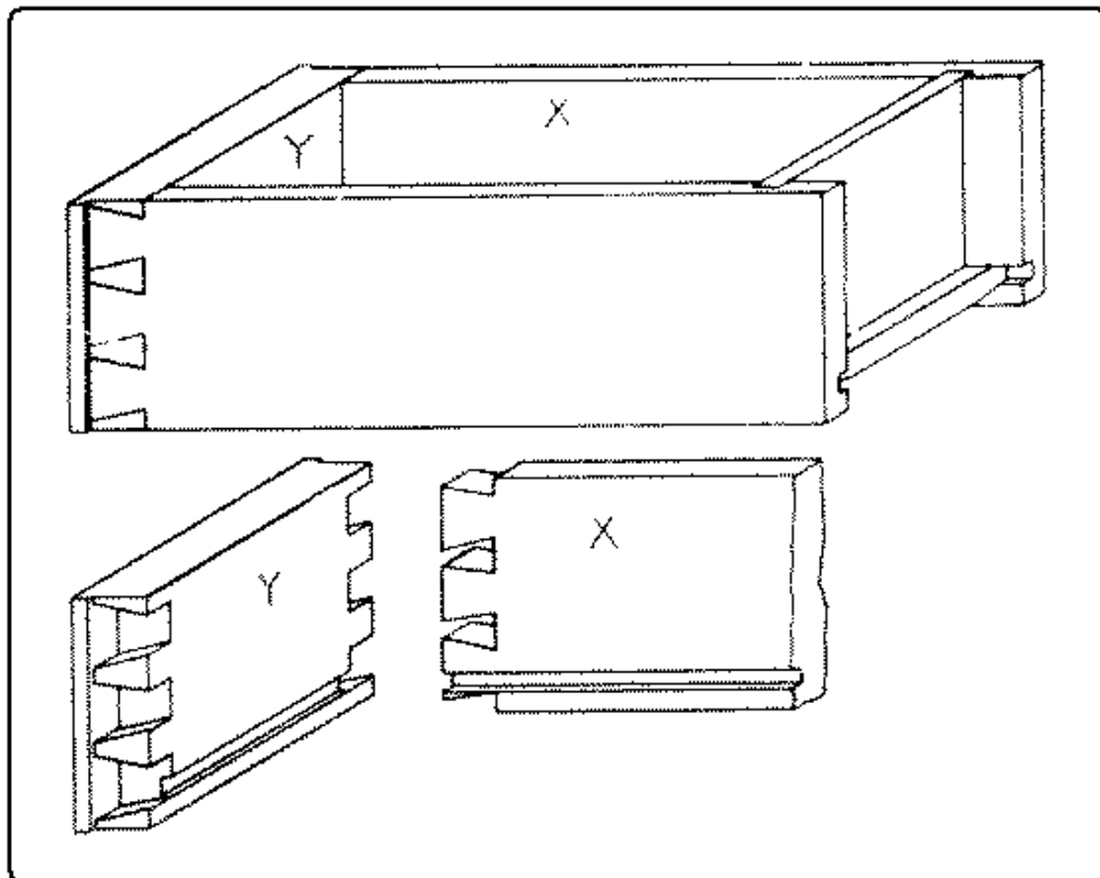
Fig. 287. Dovetailed Drawer Construction.
