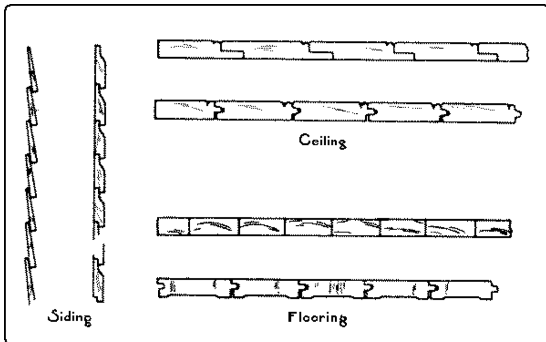
Fig. 301. Siding, Ceiling, Flooring.
