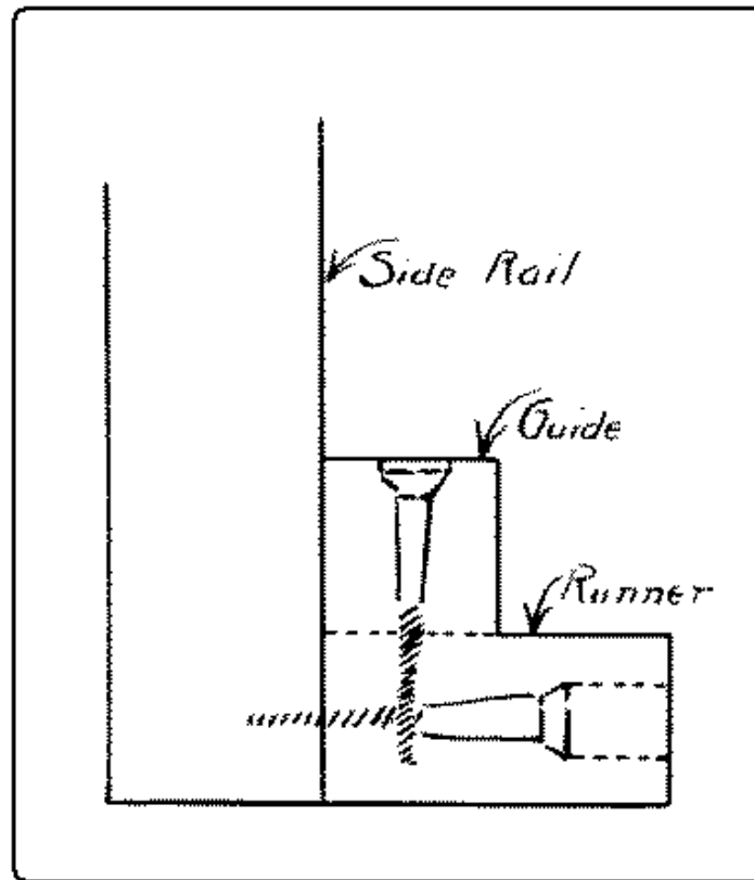
Fig. 295. Drawer Mechanism.
