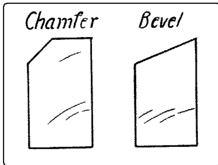
Fig. 271. Difference Between Chamfer and Bevel.
