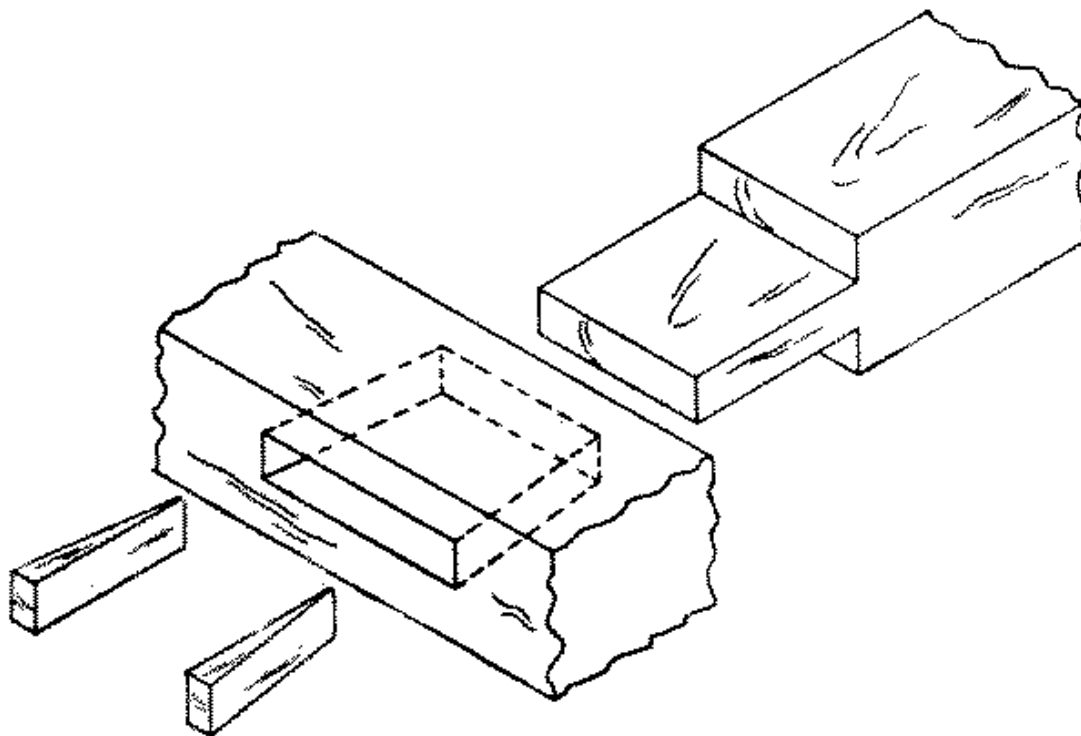
Fig. 266-34 Wedged mortise and tenon
