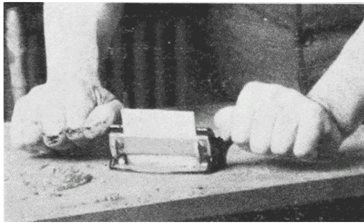
Fig. 151. Using a Veneer-Scraper.
