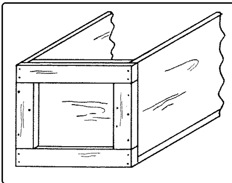
Fig. 283. Reinforced Butt Joint in Box.
