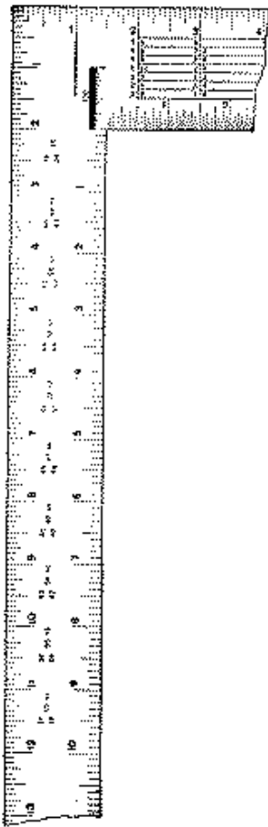
Fig. 193. Back of Steel Square, Brace Measure. Fig. 194. Face of Steel Square, Octagon, "Eight-Square," Scale.
