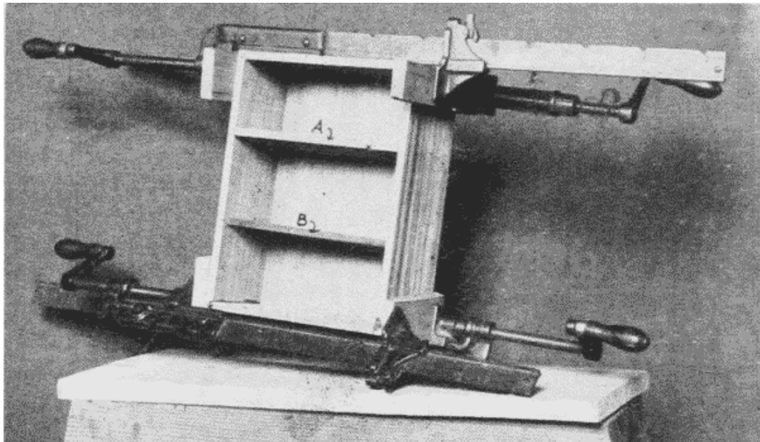
Fig. 286. Glueing Together a Box.
