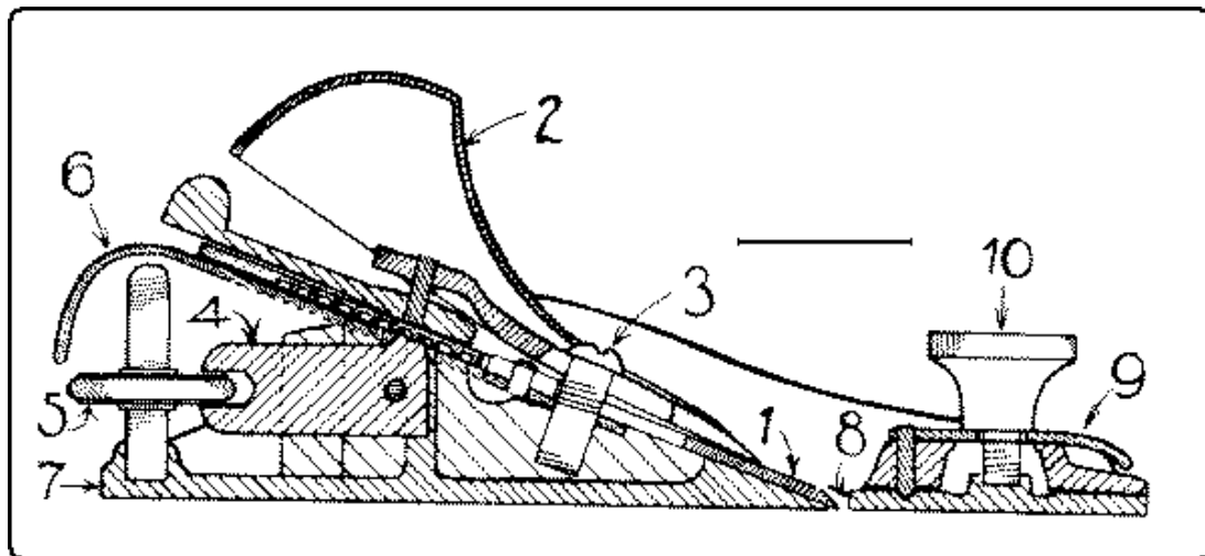
Fig. 108. Section of Block-Plane.
