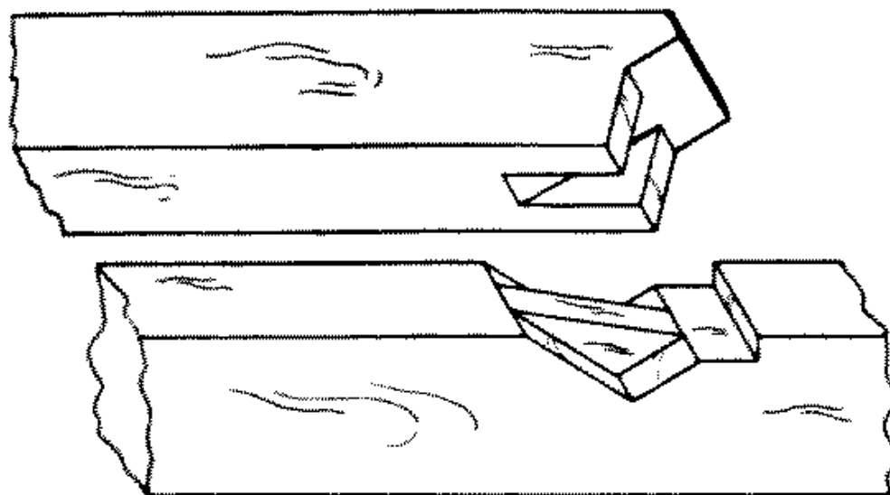
Fig. 269-68 Bridle
