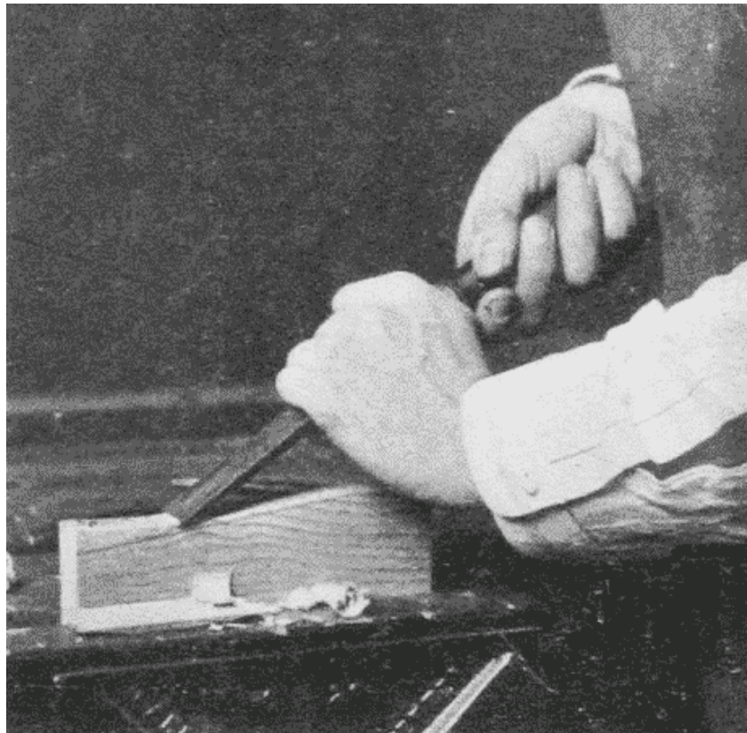
Fig. 69. Paring with a Chisel.
