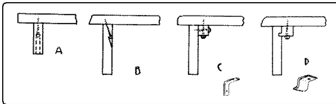
Fig. 297. Methods of attaching Table Top to Rails.
