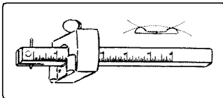
Fig. 215. Marking-Gage for Curves.
