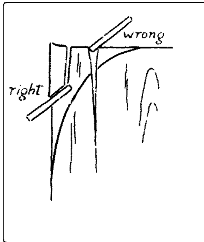
Fig. 75. Right and Wrong Ways of Perpendicular Chiseling.
