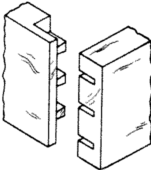
Fig. 267-50 Stopped lap dovetail
