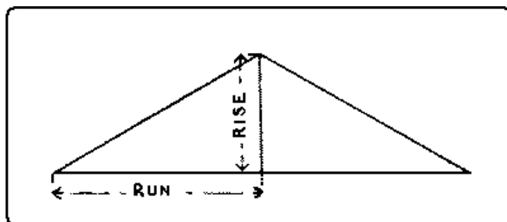
Fig. 198. The "Run" and "Rise" of a Rafter.
