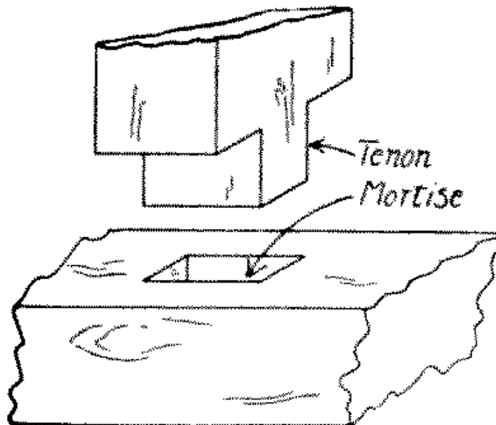
Fig. 266-30 Stub mortise and tenon
