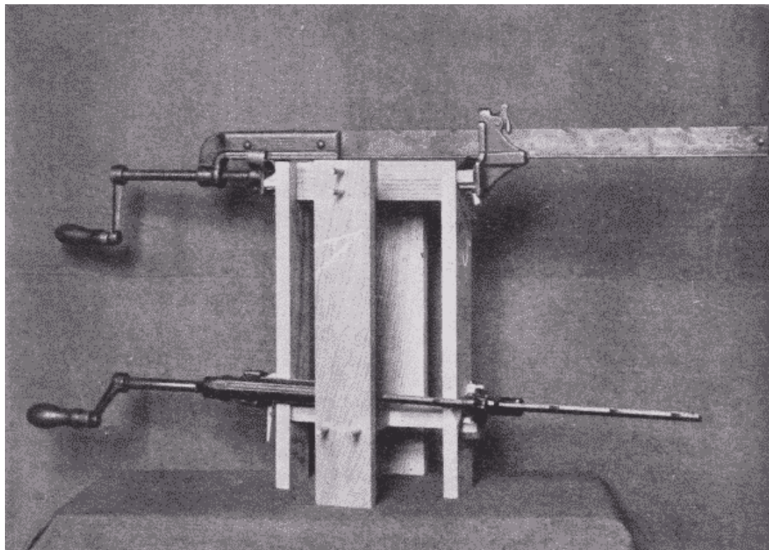
Fig. 248. Gluing-Up a Four-Legged Stand.
