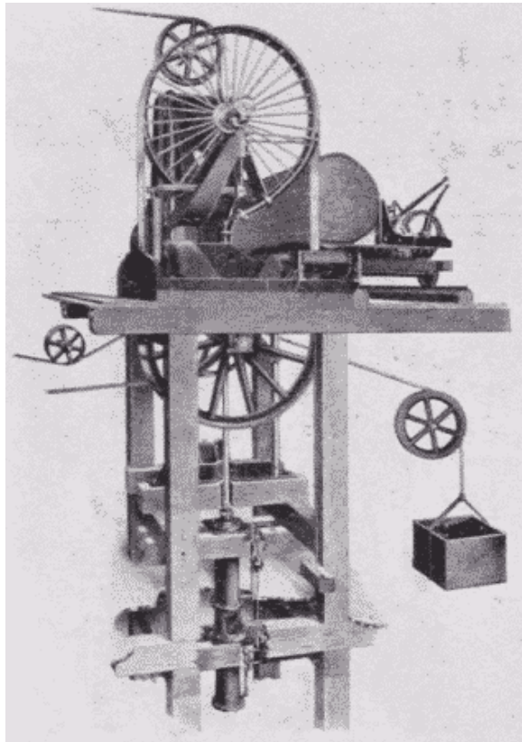
Fig. 35. Double-Carrying Telescopic Band-Mill.
