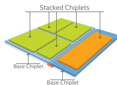
"Foveros" 3D packaging technology
